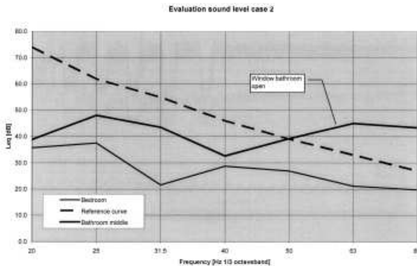
Figure 9 Evaluation of sound level in case 2.
