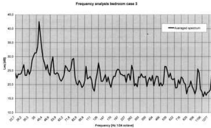
Figure 13 Averaged spectrum bedroom case 3.
